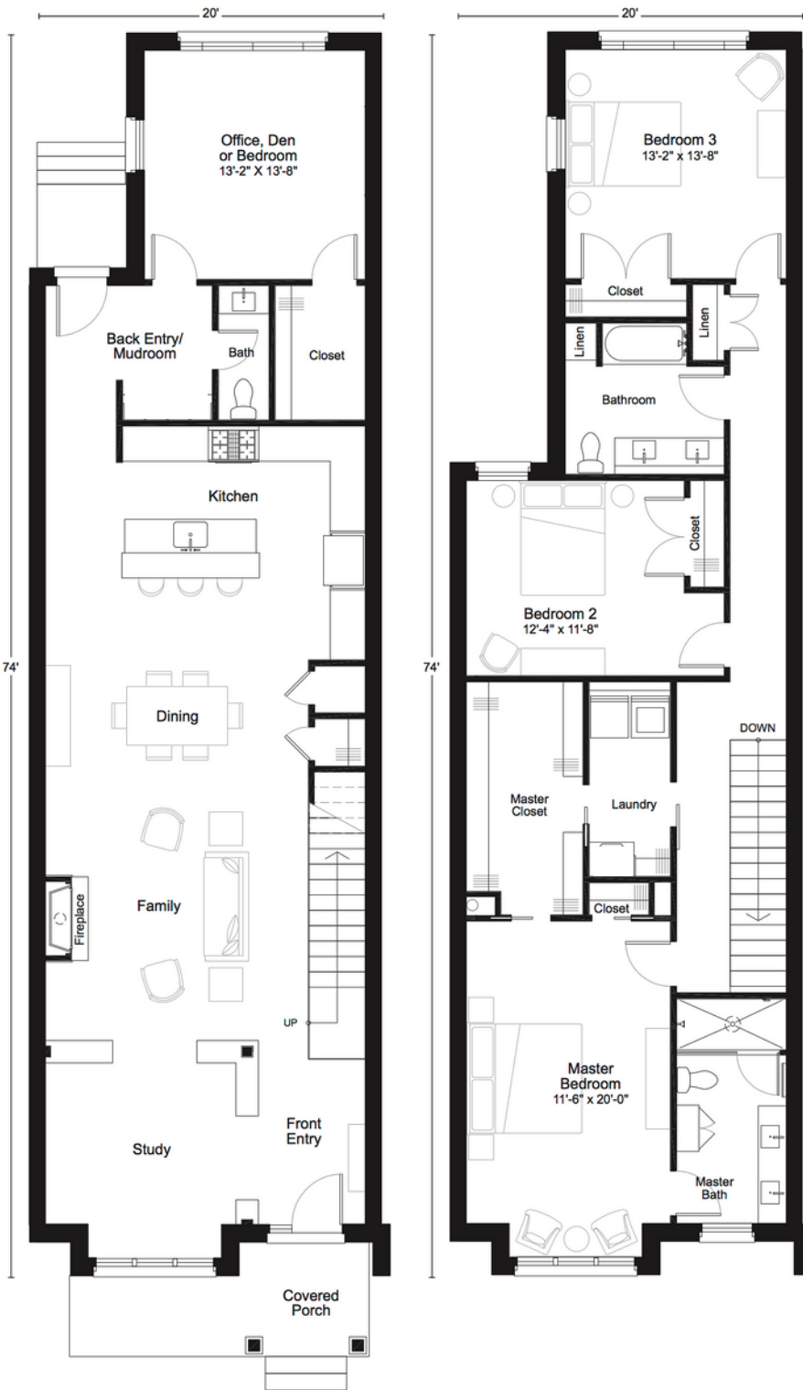
FIRST FLOOR
